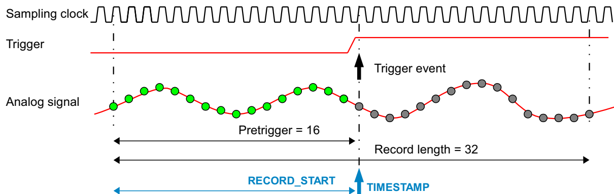
Figure 4: Pretrigger timing.
