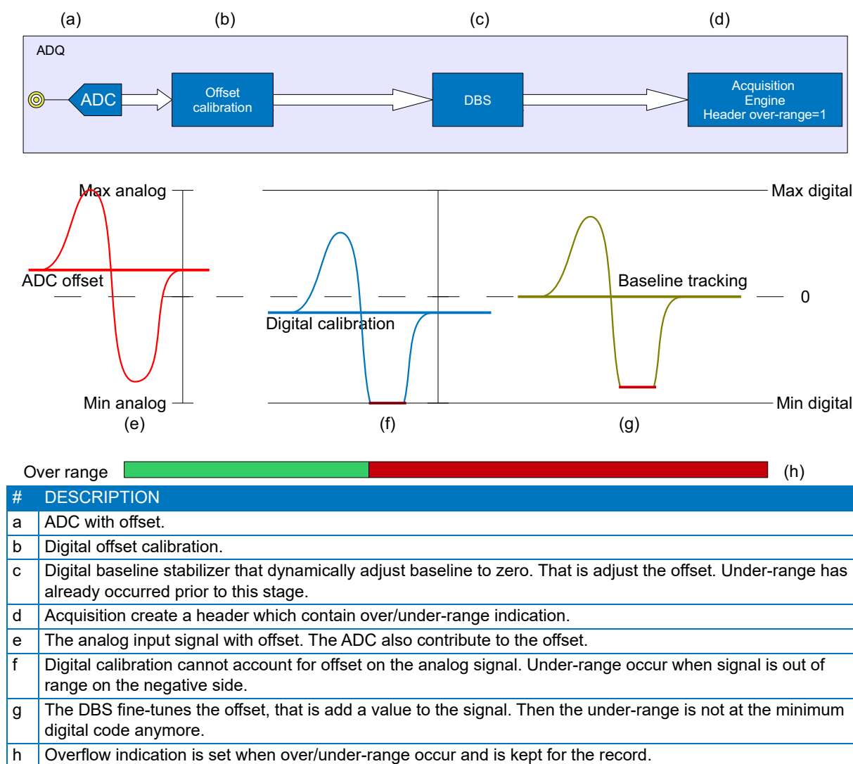
Figure 38: Under-range in the ADC calibration.
