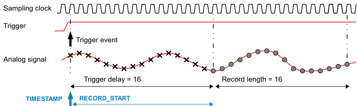
Figure 4: Pretrigger timing.
