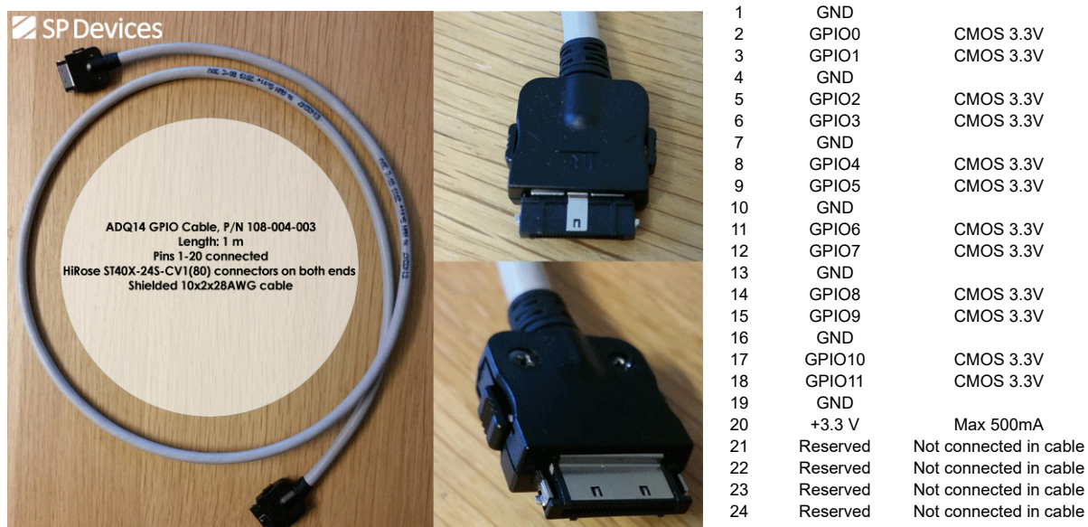
Figure 27: ADQ14 GPIO cable connection (options –GPIO, –VG and–MTCA).
