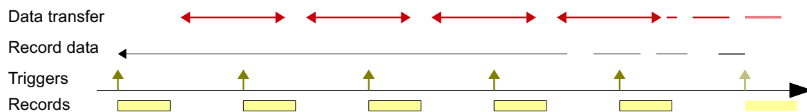
Figure 32: Multi-record timing.
