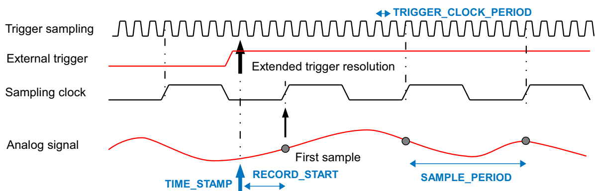
Figure 10: Extended trigger resolution timing for ADQ14-4C at 1 GSPS.
