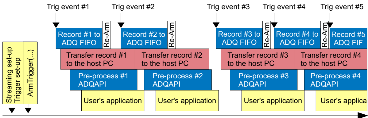
Figure 34: Timing of triggered streaming acquisition and streaming data transfer.
